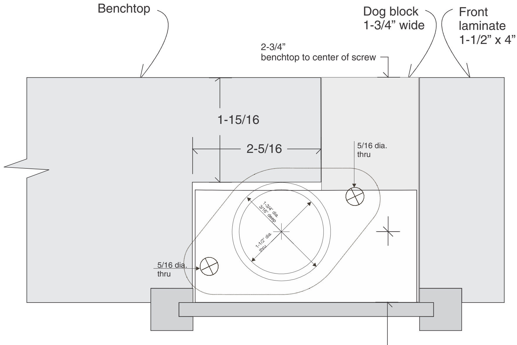
Benchcrafted Tail Vise Left Hand Installation Template v.2
